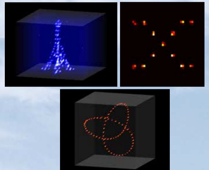
Fluorescence images of individual atoms trapped in various optical tweezers arrays. Each point corresponds to an atom.
